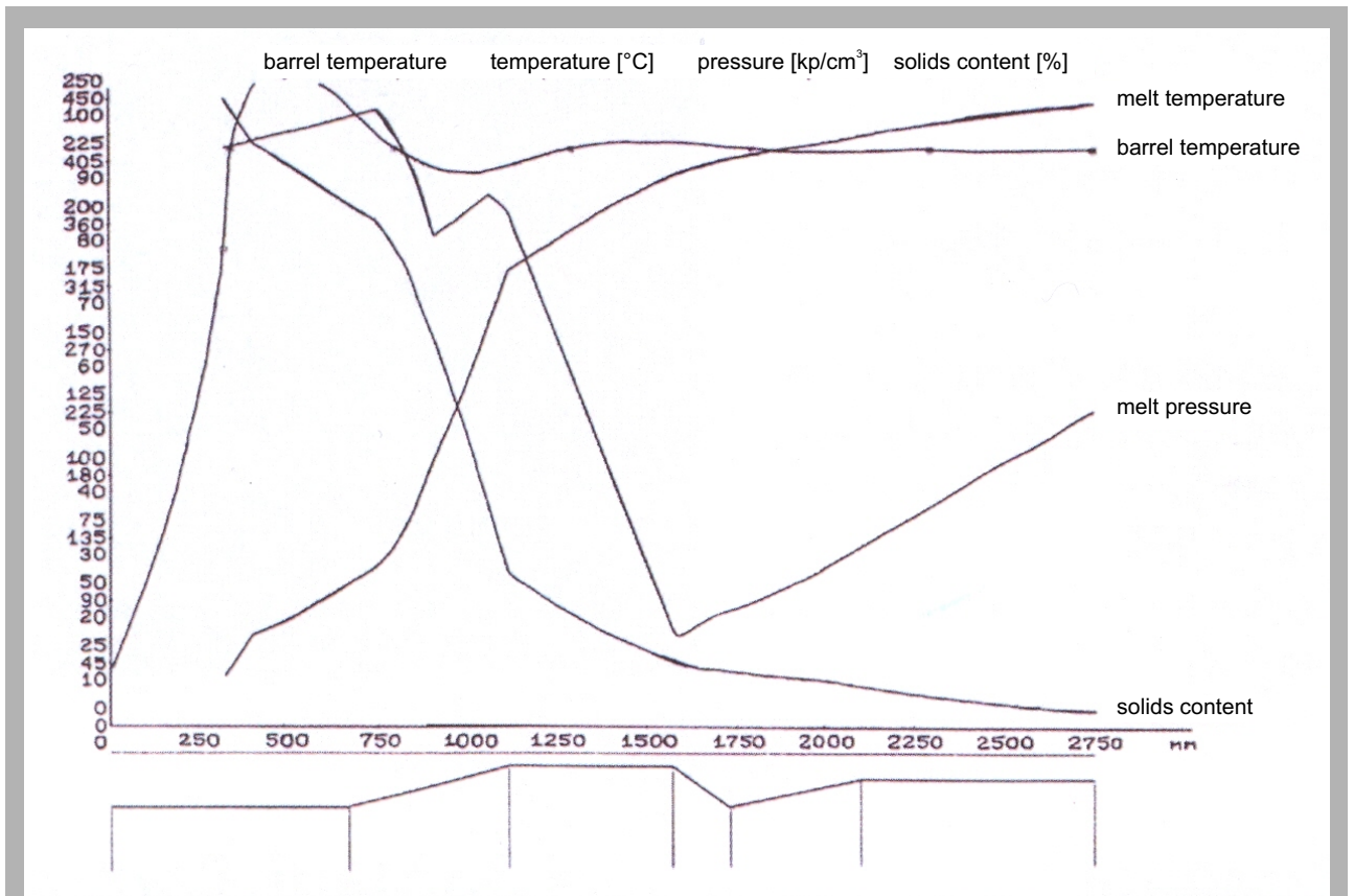
Figure: Exemplary program print-out of a vented screw
